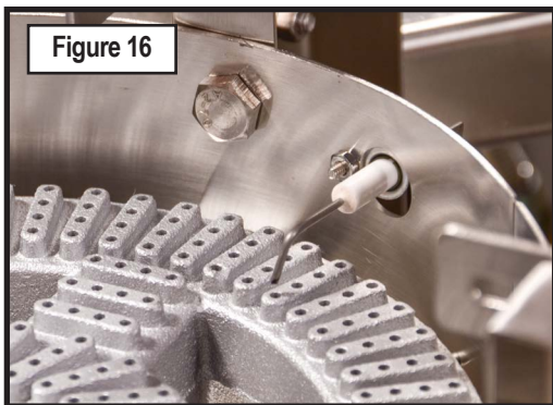
After the igniter is cut, bend the igniter so the tip is 3/16" to 1/4" from the burner casting and centered over a nozzle (Figure 16).
